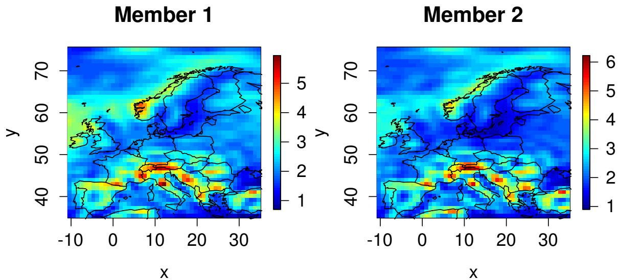
Figure 2: 3-month lead forecast for mean daily MAM precipitation (mm/d) of the NCEP's CFSv2 model for Europe considering the first two members and the period 2001-2010.
