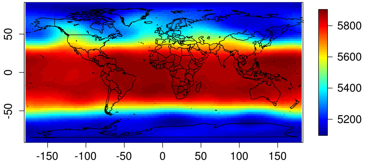
Figure 3: Global mean geopotential at surface isobaric pressure 500 mb boreal winter (DJF) of year 2010 of the NCEP-NCAR reanalysis.
